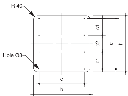
Figure 3: Placement of holes in the different types of sign plate is shown at left and the brackets at right. Values for the variable measures are given in Table 1. Details for the brackets are shown in Figure 5 and Figure 6.
